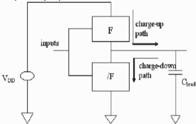
Fig. 3: A Simple Adiabatic Logic Gate
