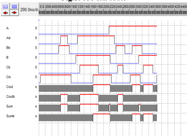
Fig.9: Simulation of 18T ALFA cell
