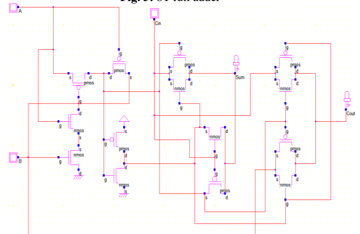
Fig.6: 14T full adder
