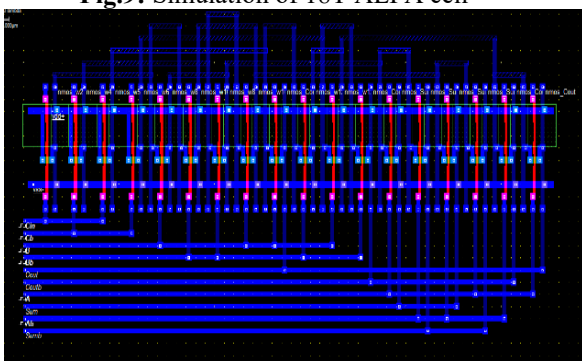
Fig.10:Layout for Proposed ALFA cell
