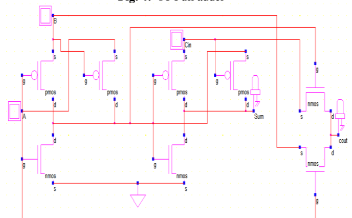
Fig. 5: 8T full adder
