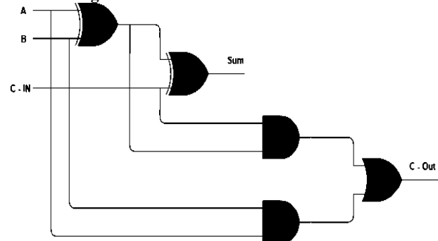
Fig.2: Full Adder logic circuit
