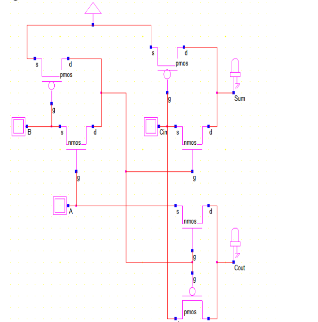
Fig. 4: 6T Full adder
