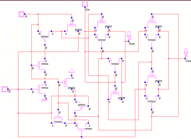
Fig.7:16T full adder
