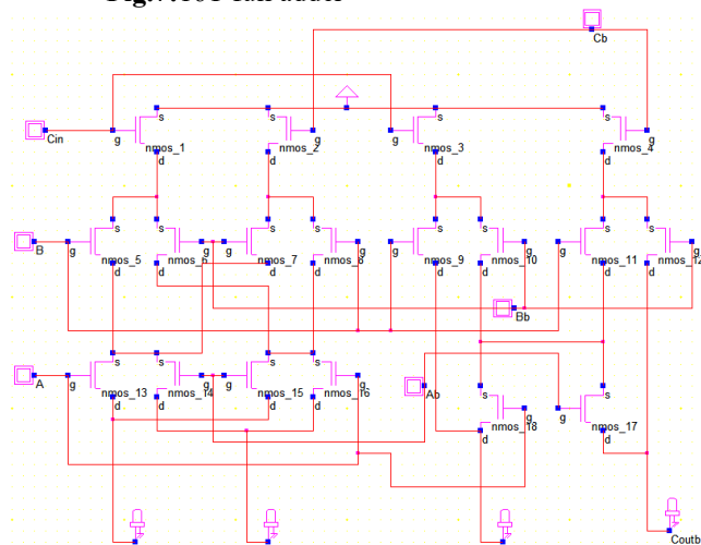
Fig.8: 18T full adder
